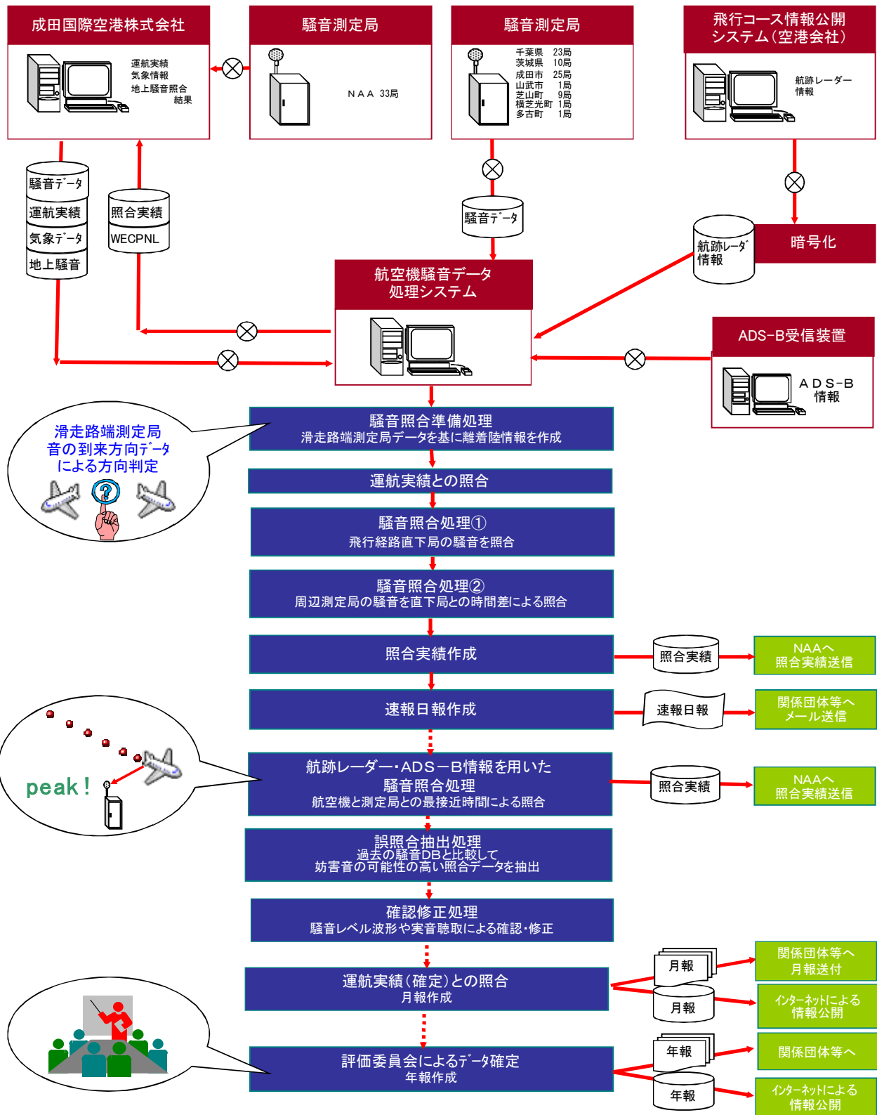
Flow chart of Aircraft Monitoring and Information Disclosure System
